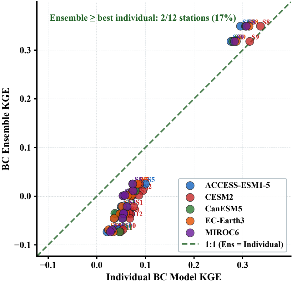
(c) Individual BC Model vs BC Ensemble — Station KGE Points above 1:1 = ensemble better | Colours = models
