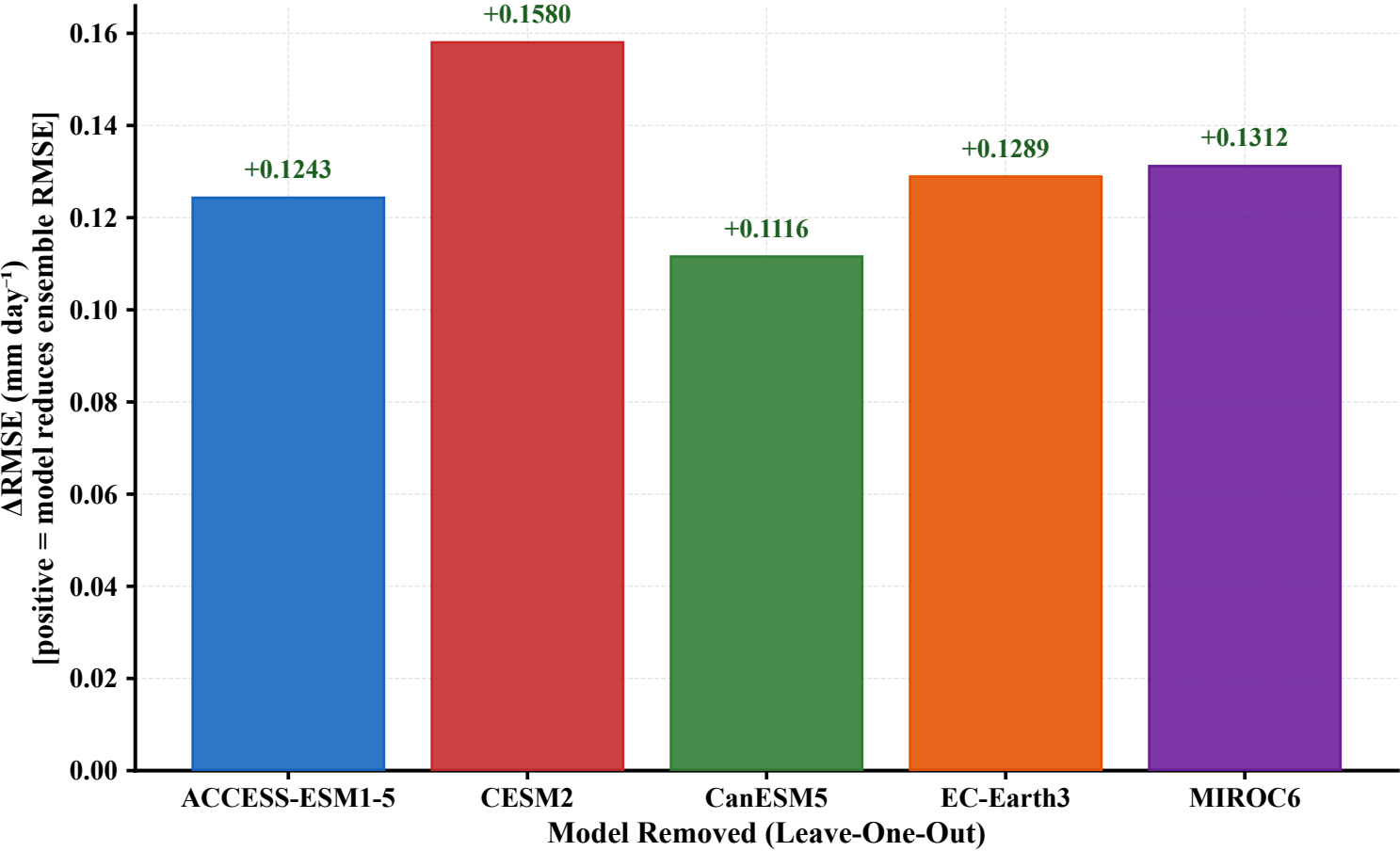
(a) Marginal Contribution — Leave-One-Out RMSE RMSE increase when model excluded from ensemble
