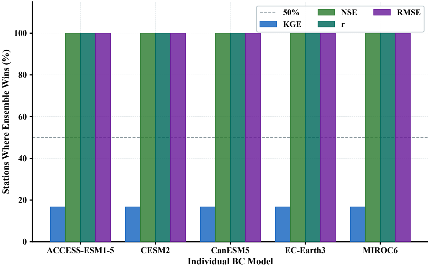
(b) Ensemble vs Individual — Win Rate % stations where BC ensemble outperforms each individual model
