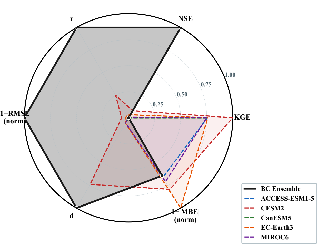
(d) Normalised Multi-Metric Radar BC Ensemble vs Individual BC Models
